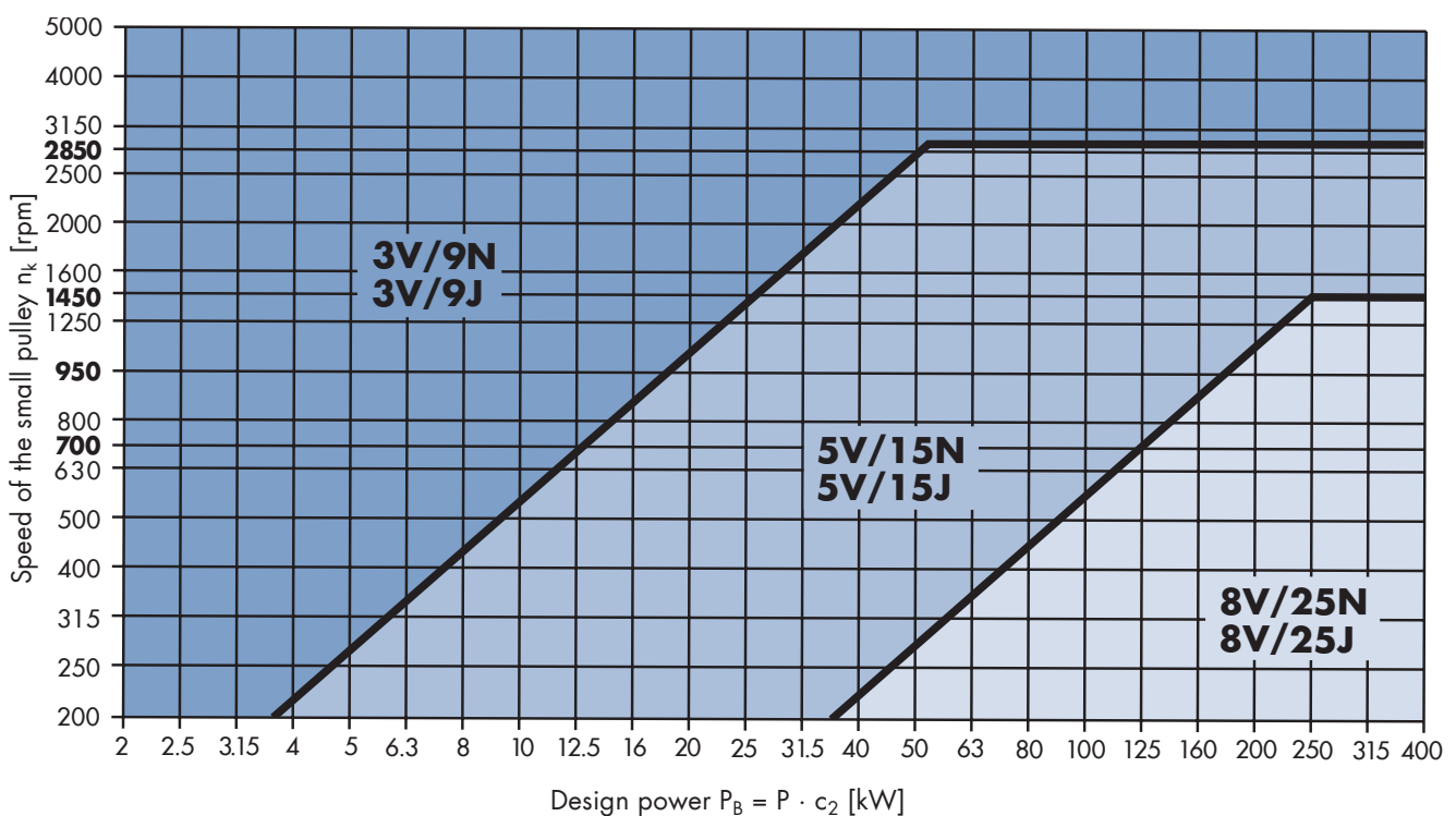
Diagram 3: optibelt SK high performance wedge belts ARPM/MPTA
