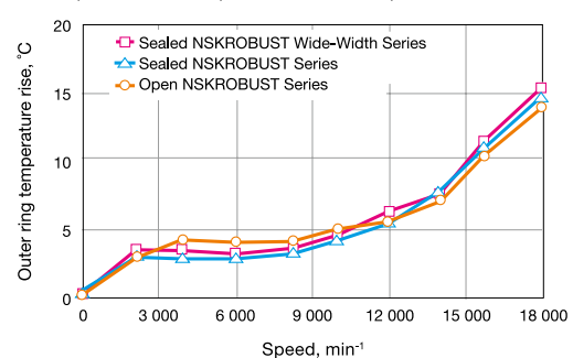
Comparison of Temperature Rise in Open vs. Sealed Bearings
